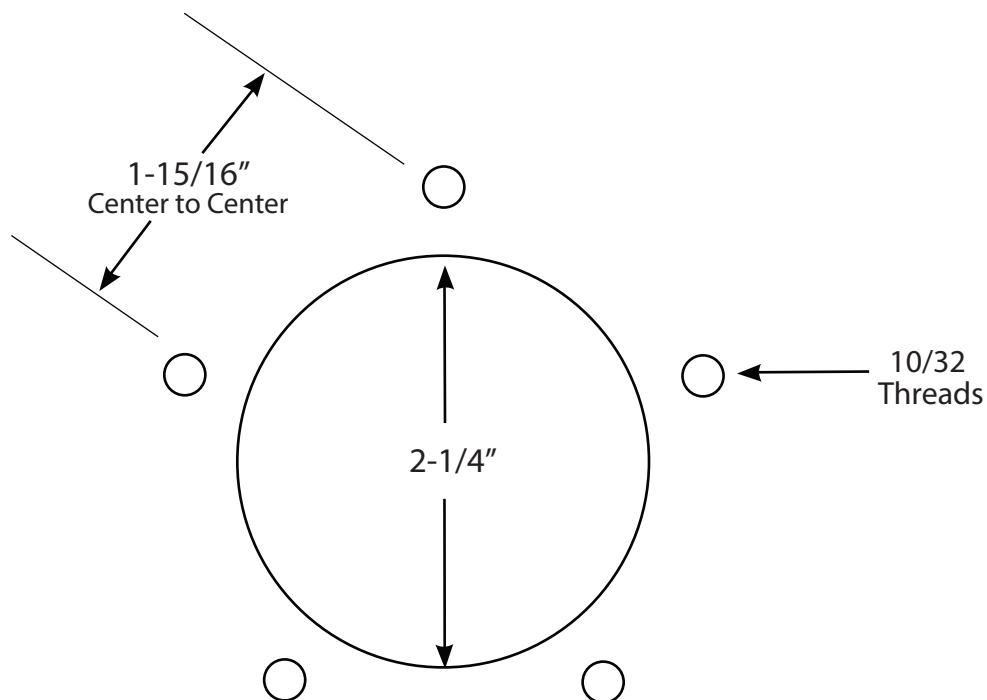
Grant 5 Bolt Pattern (Actual Size)
